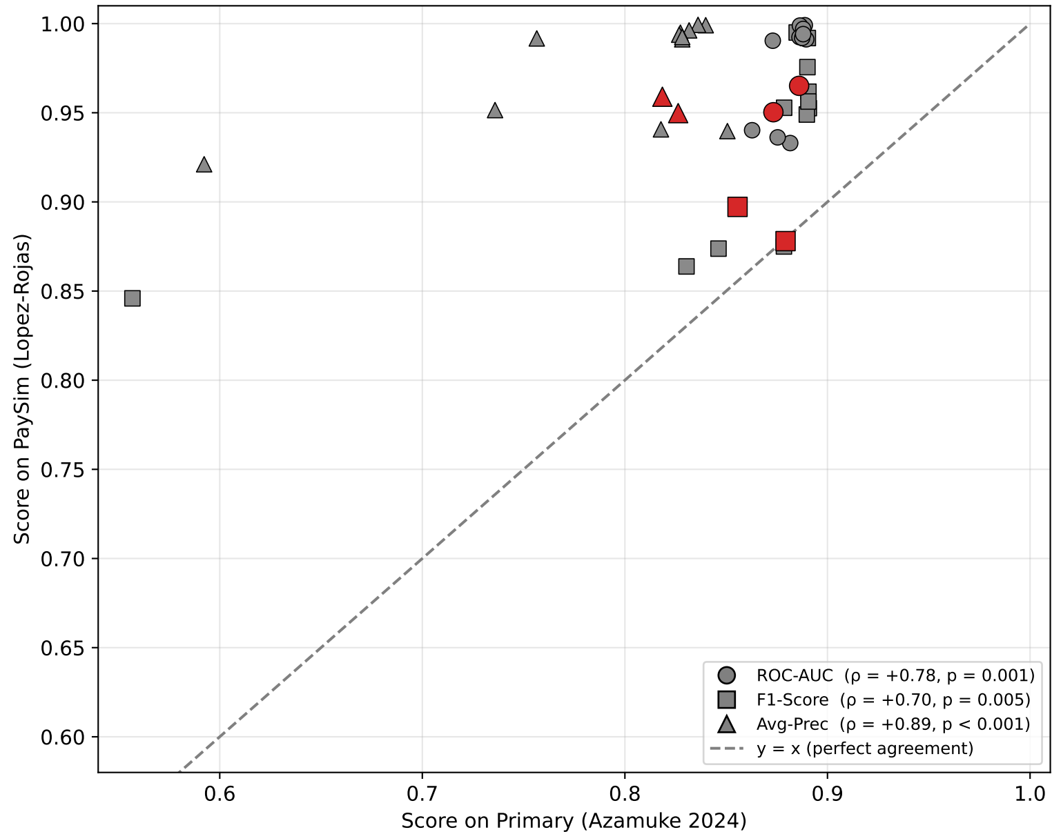
Cross-dataset score agreement (red = QDFL; o ROC-AUC, s F1, ^ Avg-Prec)
