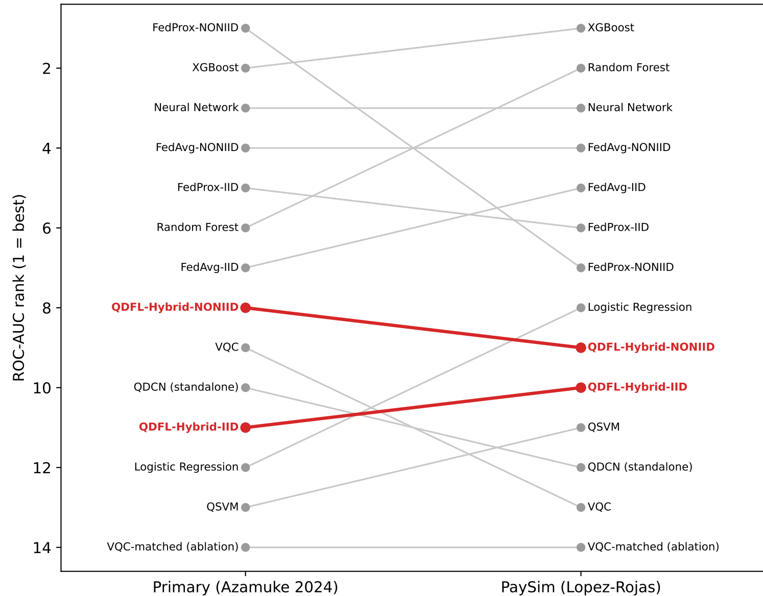
ROC-AUC rank movement across datasets (Spearman \rho = +0.78, p = 0.001 ; flat line = stable)
